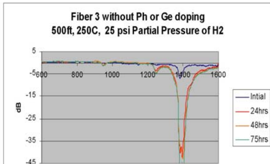
Figure 5. Here the phosphorus free fiber under test is 500 ft long. This allows more detail to be seen.
